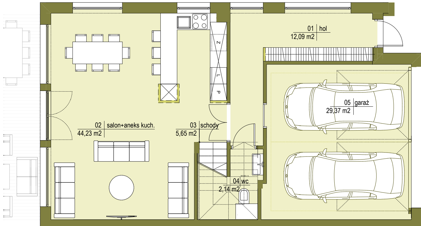
PARTER
