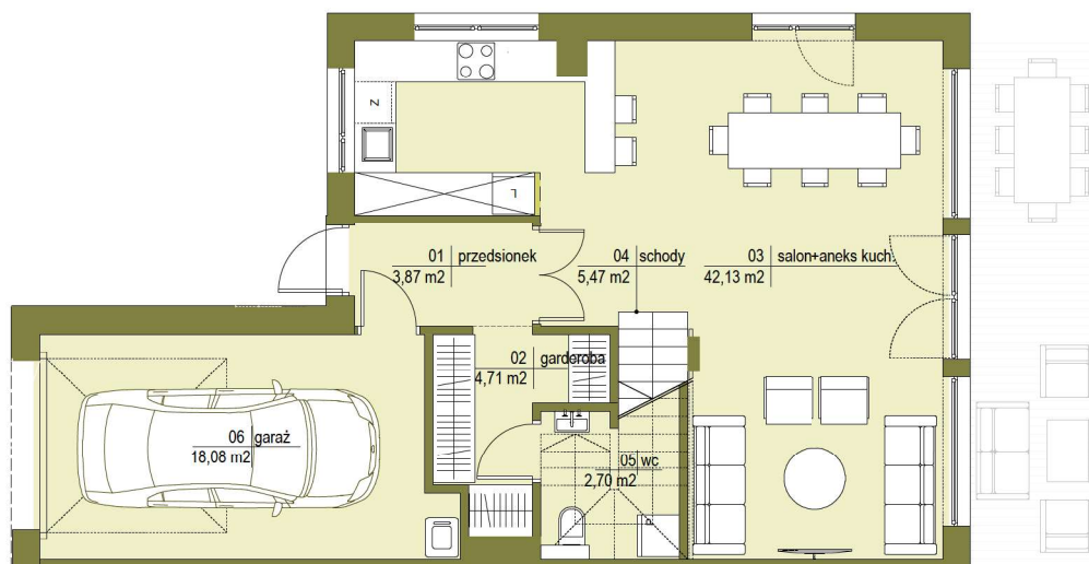
PARTER
