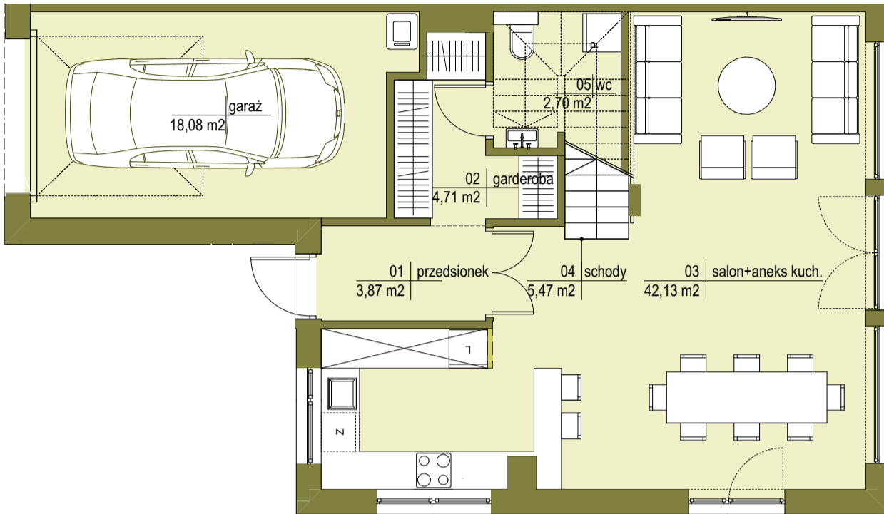
PARTER
